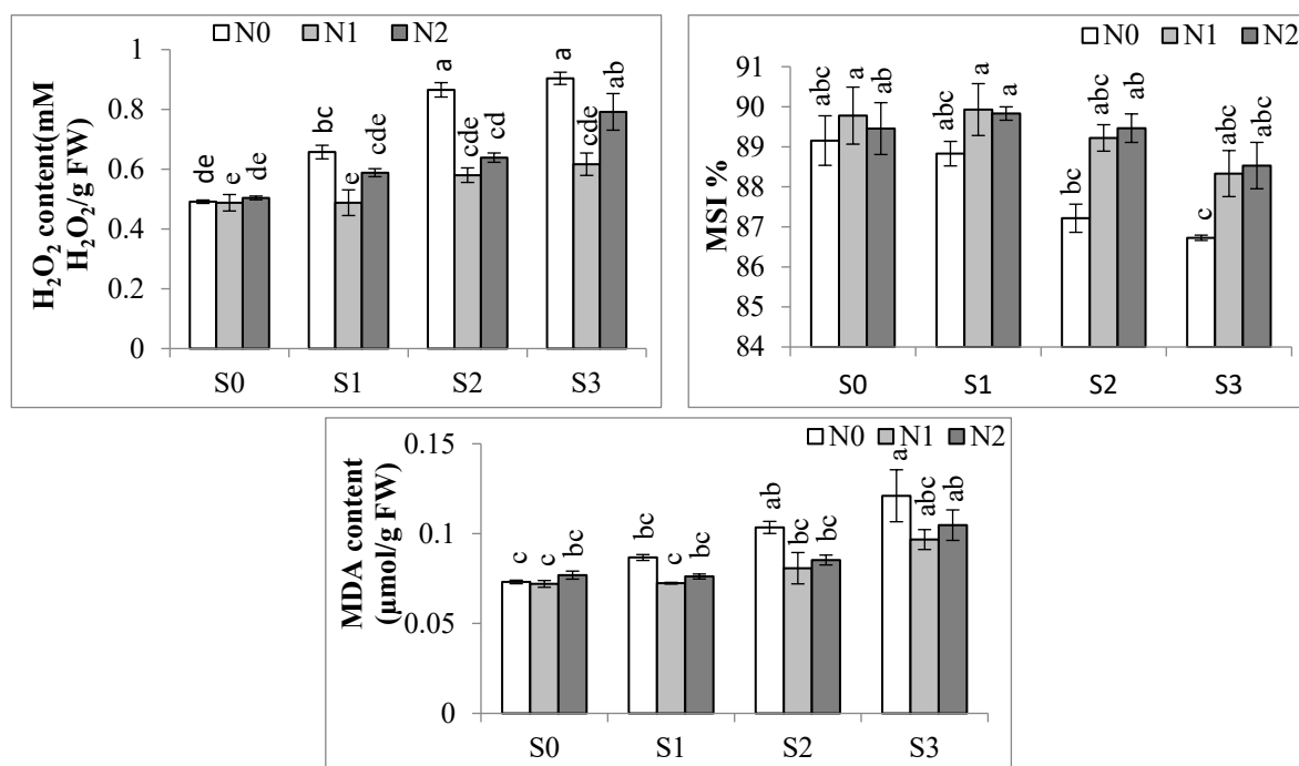
Fig. 9. Effect of Zn-chitosan NPs (N0=0 ppm, N1=100 ppm, and N2=200 ppm) foliar spraying on H_2O_2 , MDA, and MSI in spinach shoots under soil salinity stress. S0 = control, S1=3 ds/m, S2 = 5 ds/m and S3 = 7 ds/m.
