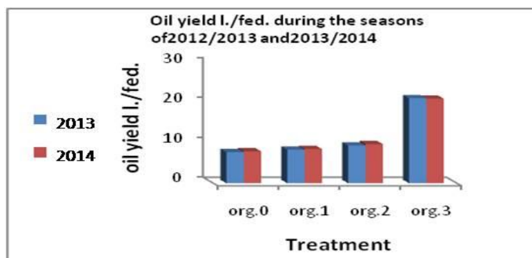
Figure 1: Effect of different rates of cattle manure on oil yield litre/fed. of cumin.
